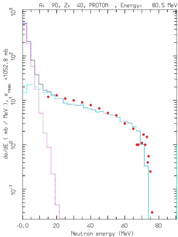
Example of angle integrated ^{90}\text{Zr}(p,xn) at 80.5 MeV calculations with the full algorithm (right), and without the INC stage (left). The various lines show the total, INC, preeq. and evaporation contributions, the exp. data have been taken from M.Trabandt et al. PRC39 (1989) 452
