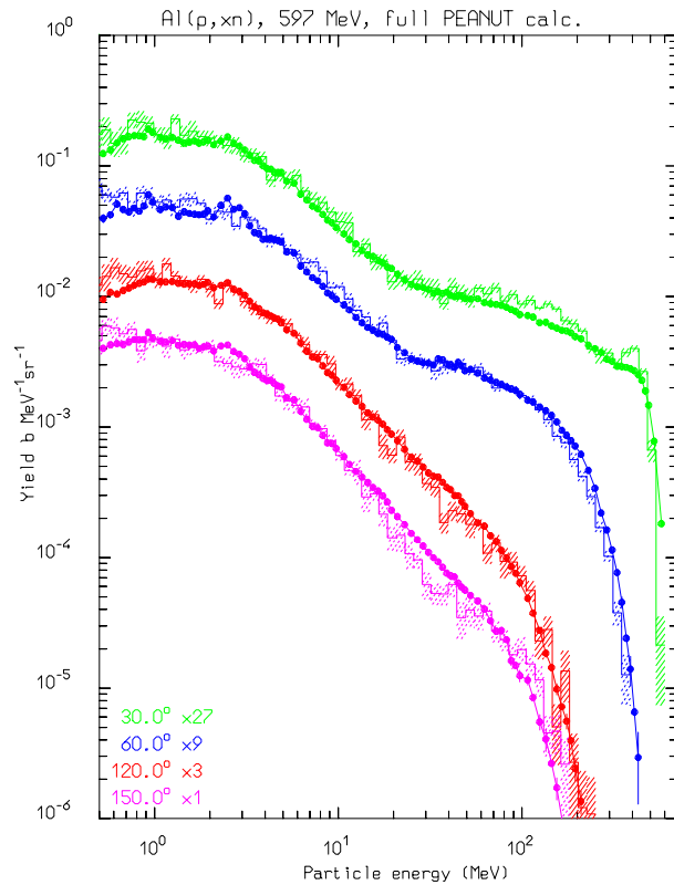
Computed (histograms) and experimental (symbols) double differential neutron distributions for Al(p,xn) (left) at 597 MeV and Pb(p,xn) at 3 GeV. The exp. data have been taken from W.B. Amian et al., Nucl. Sci. Eng. 115 , (1993) 1, and K. Ishibashi et al, Nucl. Sci. Technol. 32 (1995) 827.
