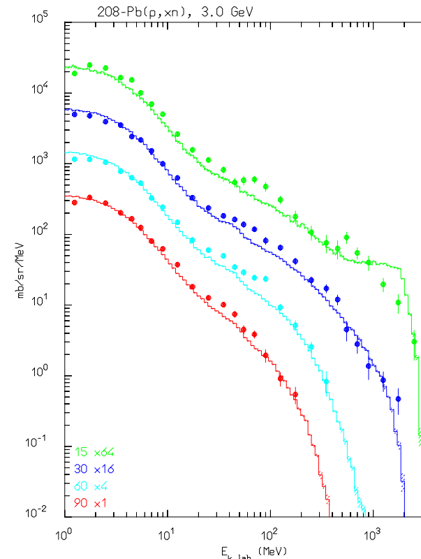
Computed (histograms) and experimental (symbols) double differential neutron distributions for Al(p,xn) (left) at 597 MeV and Pb(p,xn) at 3 GeV. The exp. data have been taken from W.B. Amian et al., Nucl. Sci. Eng. 115 , (1993) 1, and K. Ishibashi et al, Nucl. Sci. Technol. 32 (1995) 827.
