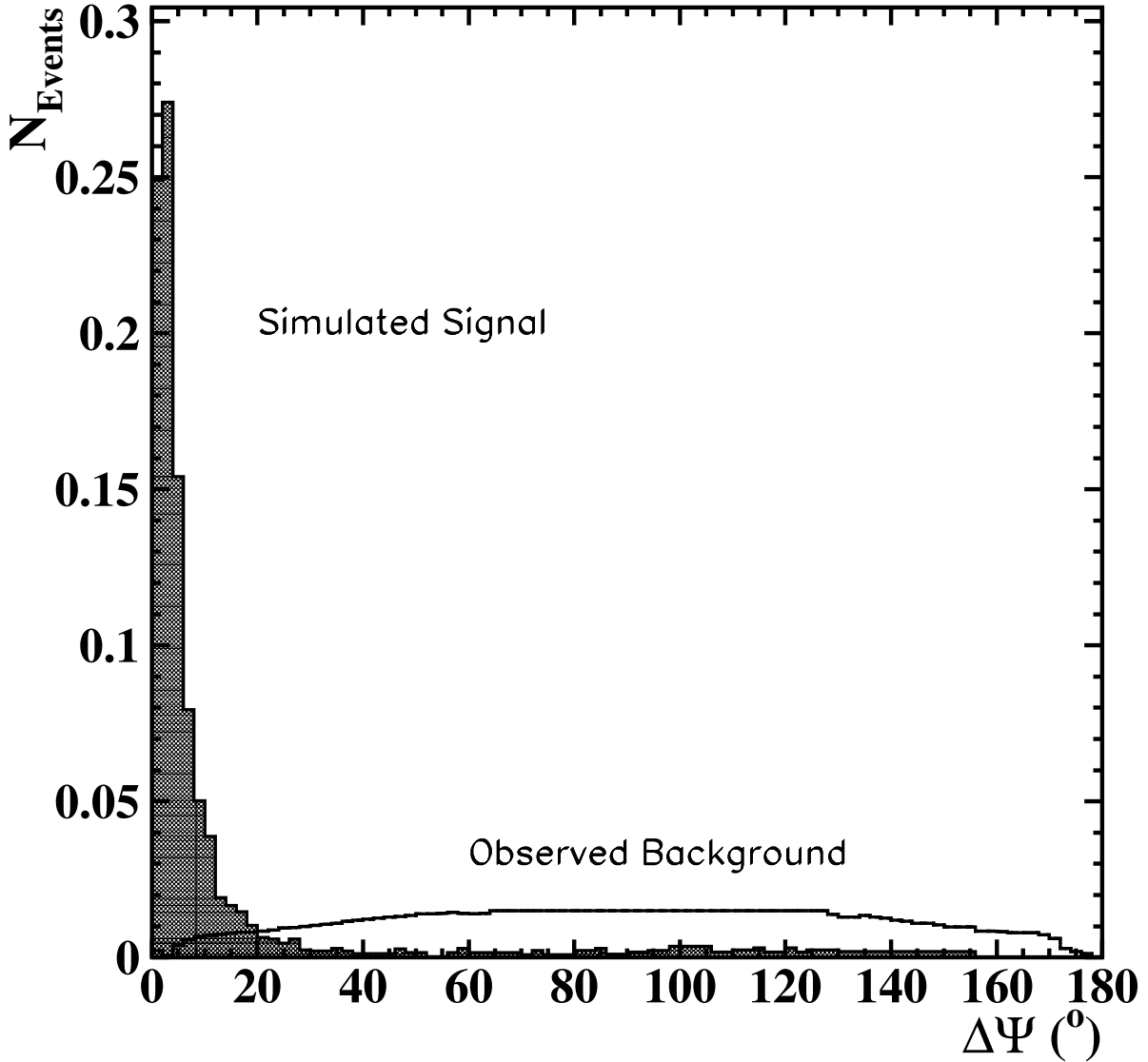
Fig. 5.— The expected distribution of angular mismatch \Delta\Psi_1 for a simulated muon neutrino spectrum (shaded region) and observed background (open region). \Delta\Psi_1 = 0 is the position of the burst determined from photon observations. Selecting events with \Delta\Psi_1 \leq 12^{\circ} retains more than 90% of the signal events.
