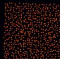
WIMPs created early in the big bang
