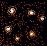
Galaxies continue to evolve
