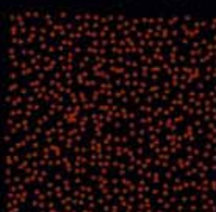
They decay to fast super-WIMPs
