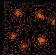
They slow down and seed galaxies
