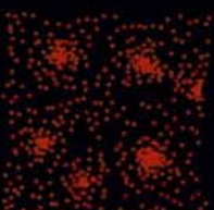
Super-WIMPs slow down and seed galaxies
